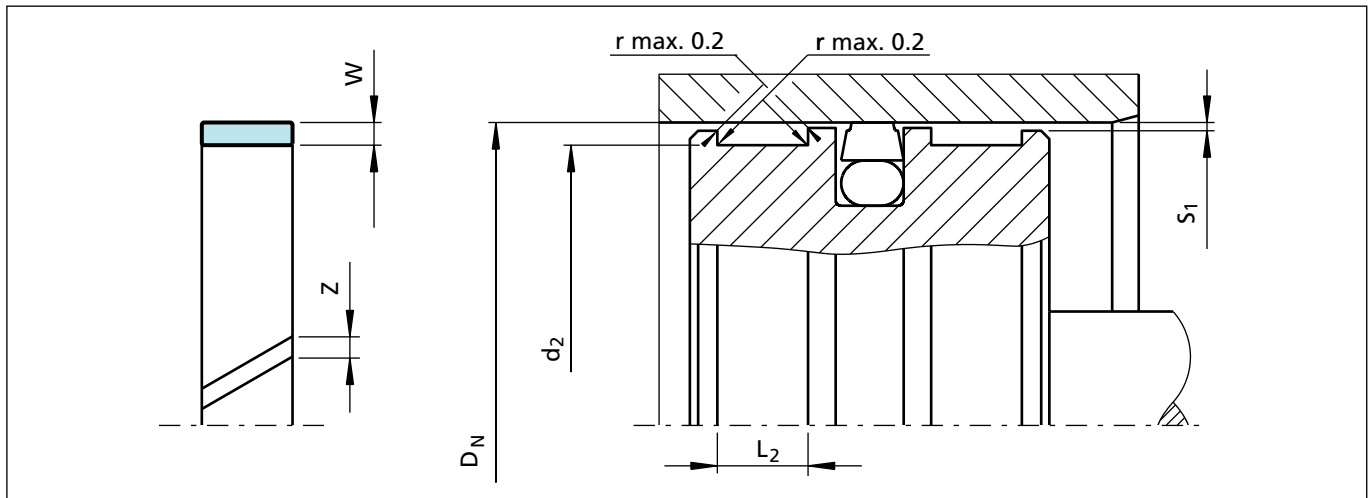
Figure 9 Installation drawing
