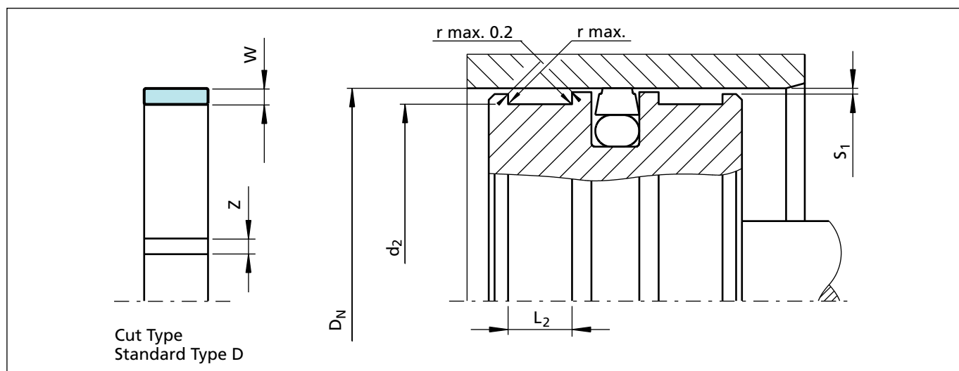
Figure 12 Installation drawing
